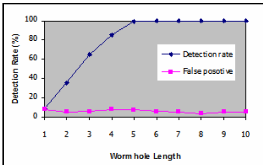
Fig. 4. Detection Rate
