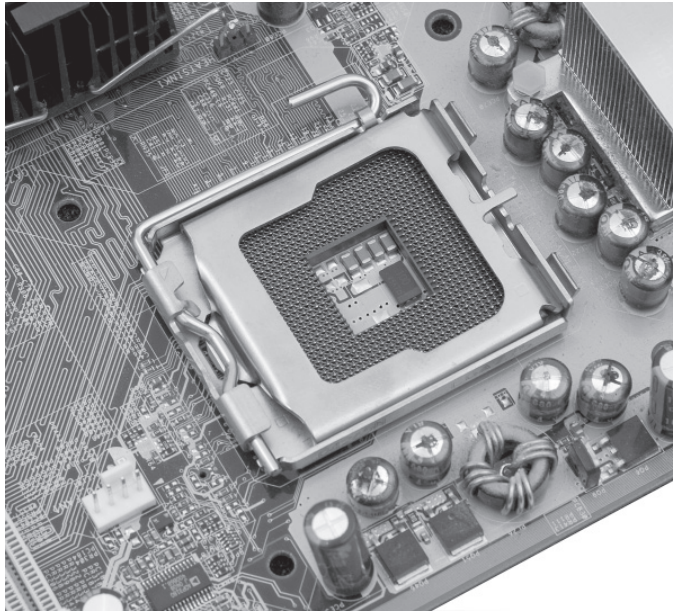
Figure 3-24 ZIF socket with cage over the top
