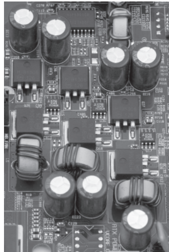
Figure 3-37 Typical motherboard voltage regulators
