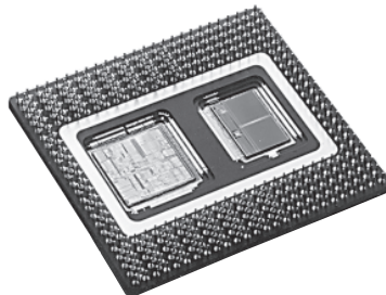
Figure 3-41 A P6 opened to show separate CPU and L2 cache (Photo courtesy Intel Corp)
