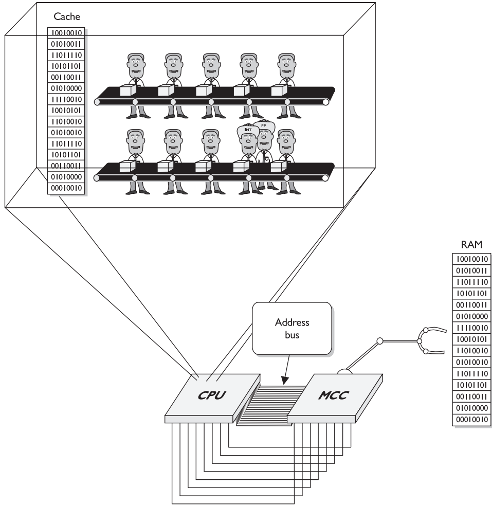
Figure 3-33 RAM cache
