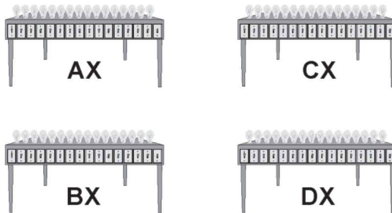
Figure 3-6 The four general-purpose registers
