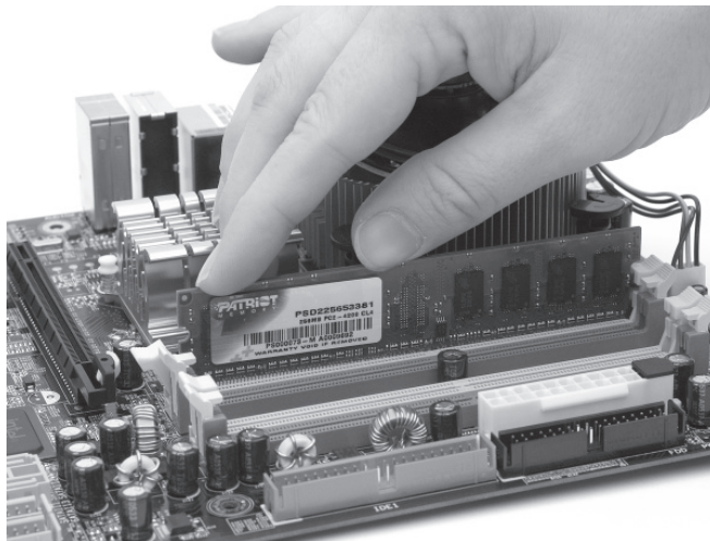
Figure 4-28 Inserting a DIMM
