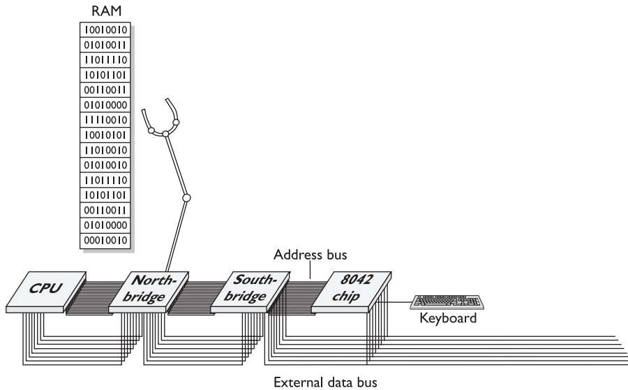
Figure 5-5 Electronic view of the keyboard controller
