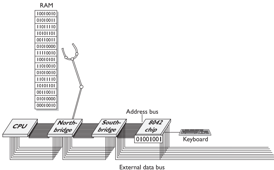
Figure 5-6 Scan code stored in keyboard controller's register
