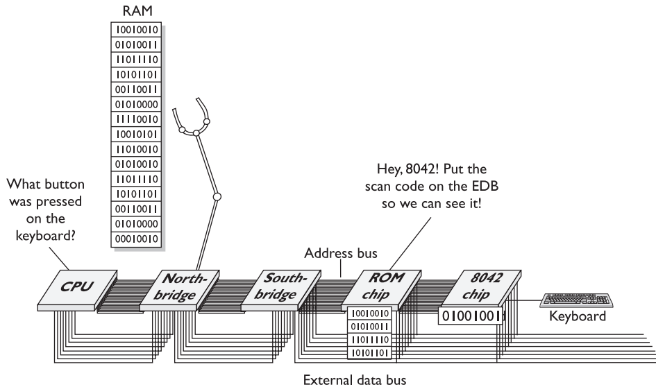
Figure 5-10 CPU running BIOS service
