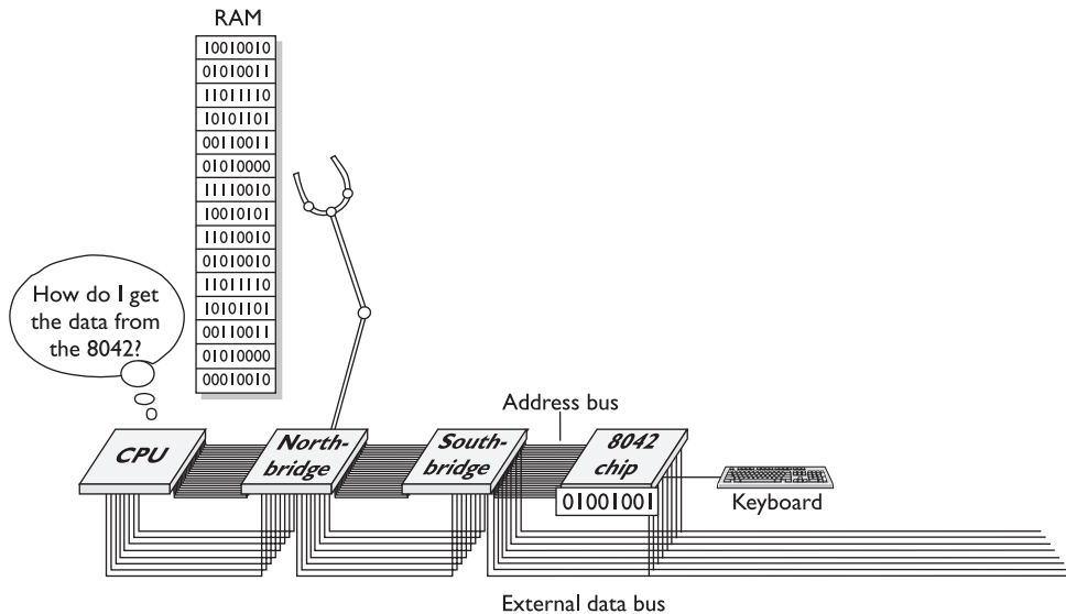
Figure 5-7 The CPU ponders its dilemma....
