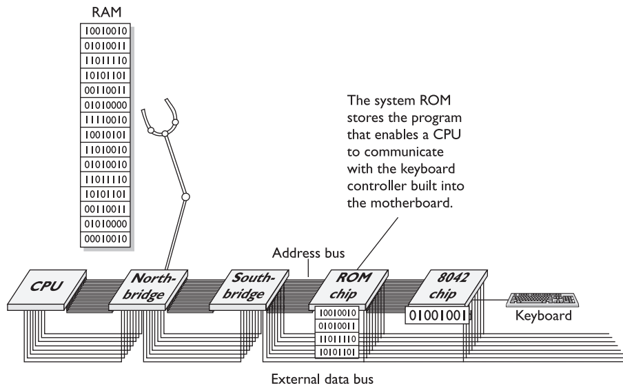
Figure 5-9 Function of the Flash ROM chip
