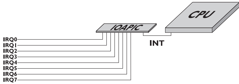
Figure 6-18 Eight interrupt wires (IRQs) run from the expansion bus to the IOAPIC.
