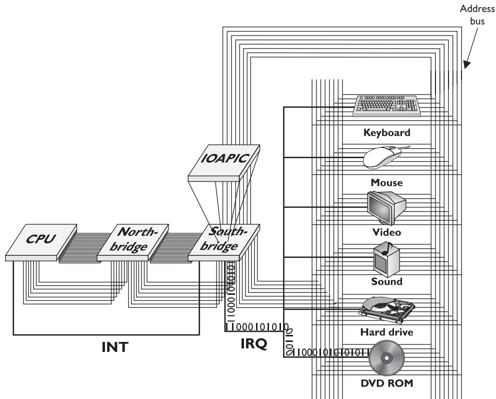
Figure 6-19 IOAPIC at work
