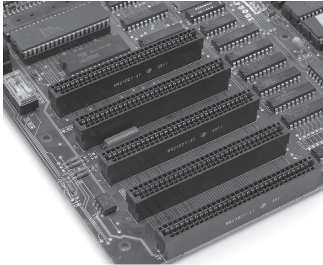
Figure 6-6 Eight-bit PC/XT slots
