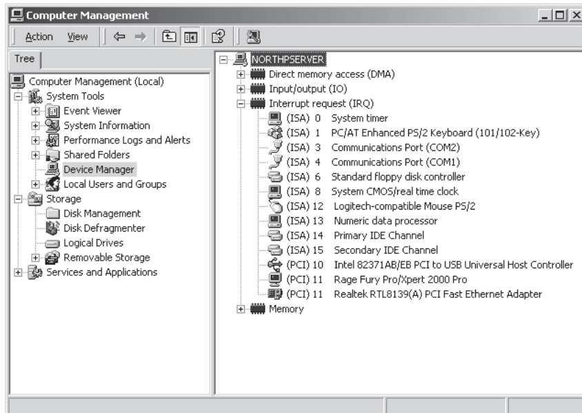
Figure 6-21 IRQs in a PIC system
