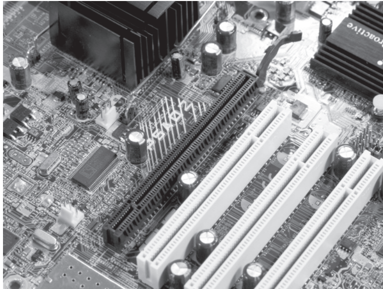
Figure 6-12 PCIe \times 16 slot (black) with PCI slots (white)
