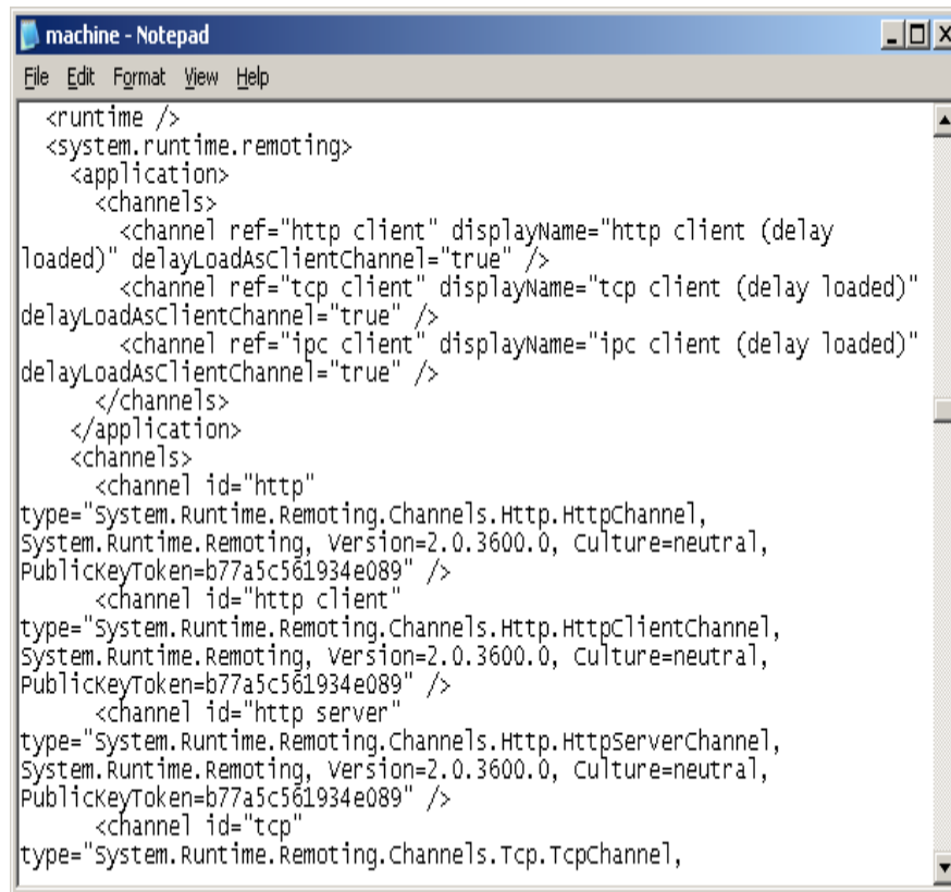
Figure :- 4.6 Channels and Formatter in machine.config file
