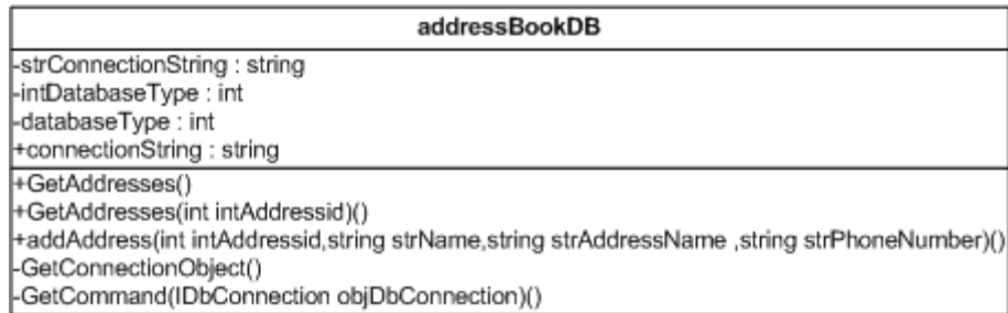
Figure 15.21 : - Database access layer diagram
