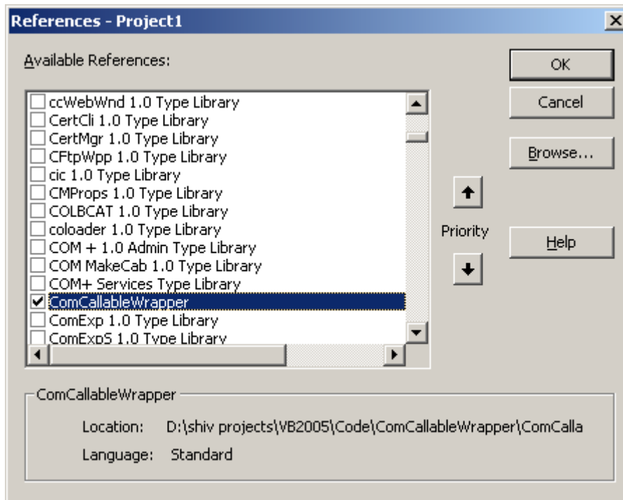
Figure :- 2.2 VB6 IDE referencing the CCW
