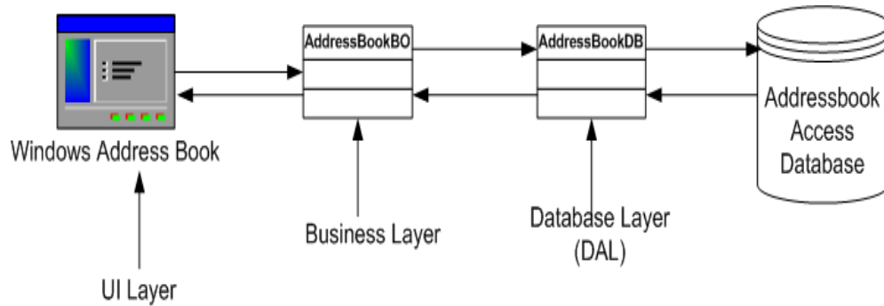
Figure 15.19 : - Architecture road map for address book application
