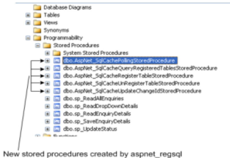
Figure 5.2 : - New stored procedures created
