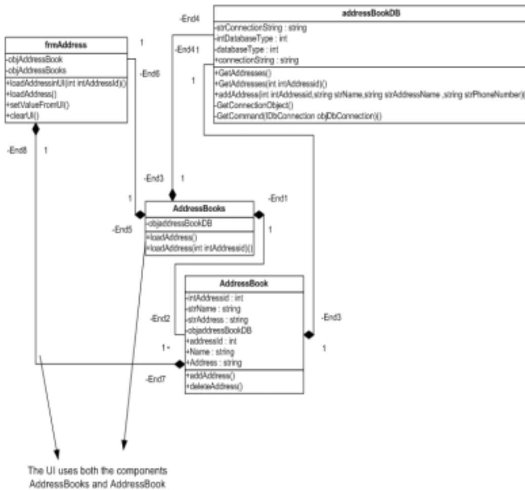
Figure 15.23 : - UI component Diagram
