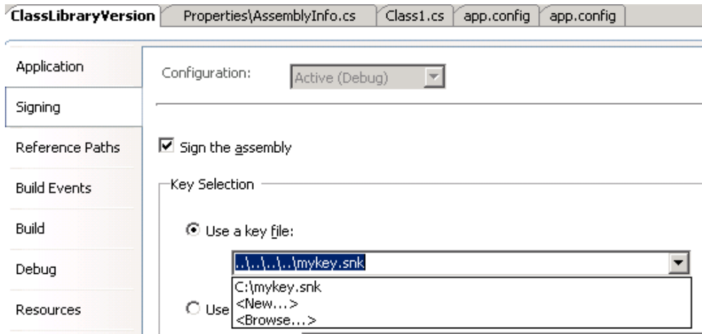
Figure 1.13 : - Strong naming your DLL
