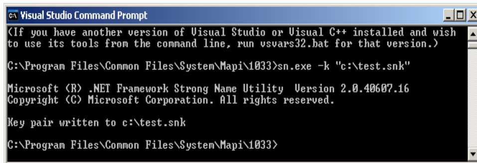
Figure :- 1.5 Successful output of SN.EXE
