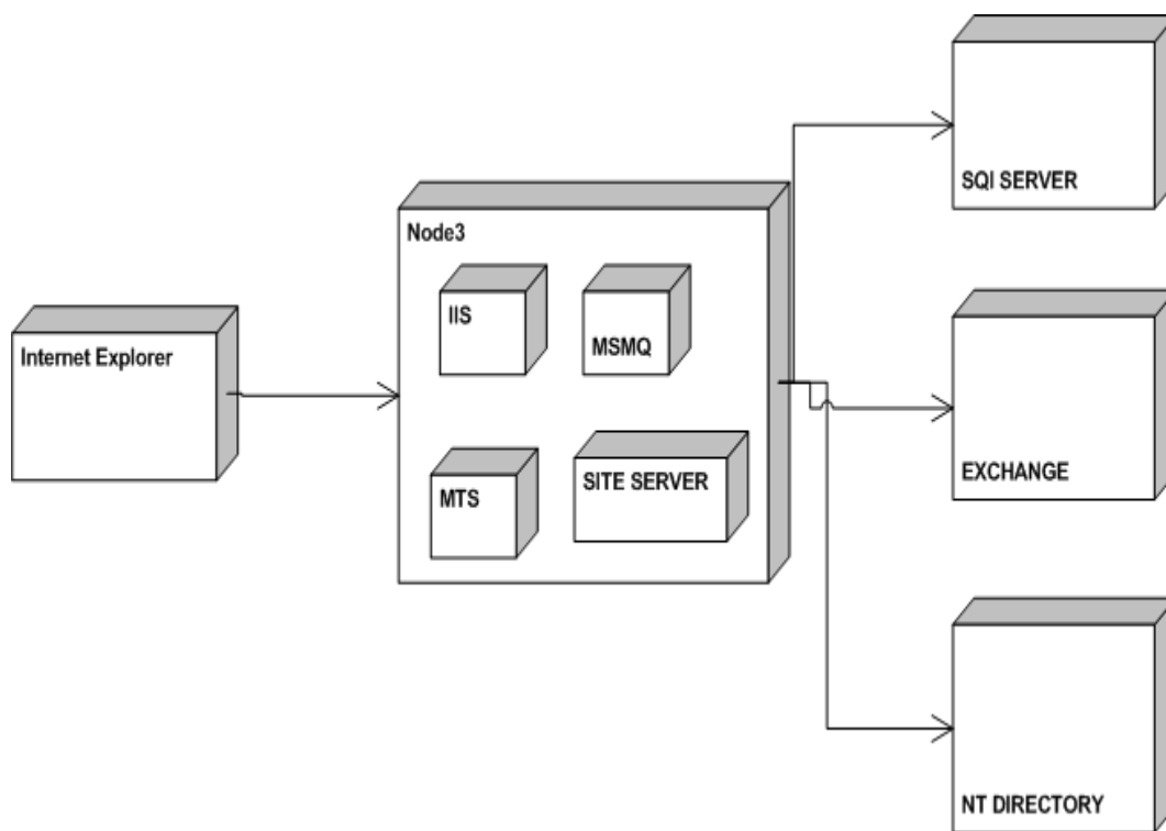
Figure :- 8.6 Windows DNA sections
