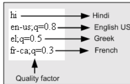
Figure 14.8 : - Output from request.Userlanguages
